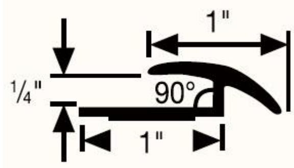
168-XX Smooth Carpet-to-Tile Transition
